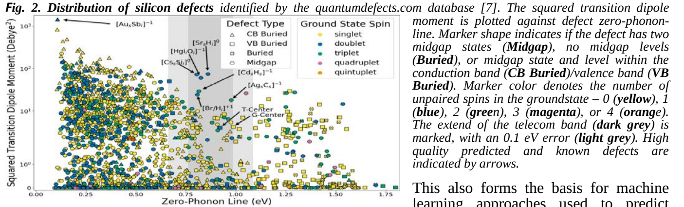
Fig. 2. Distribution of silicon defects identified by the quantumdefects.com database [7]. The squared transition dipole moment is plotted against defect zero-phonon-line. Marker shape indicates if the defect has two midgap states (Midgap), no midgap levels (Buried), or midgap state and level within the conduction band (CB Buried)/valence band (VB Buried). Marker color denotes the number of unpaired spins in the groundstate – 0 (yellow), 1 (blue), 2 (green), 3 (magenta), or 4 (orange). The extend of the telecom band (dark grey) is marked, with an 0.1 eV error (light grey). High quality predicted and known defects are indicated by arrows.
