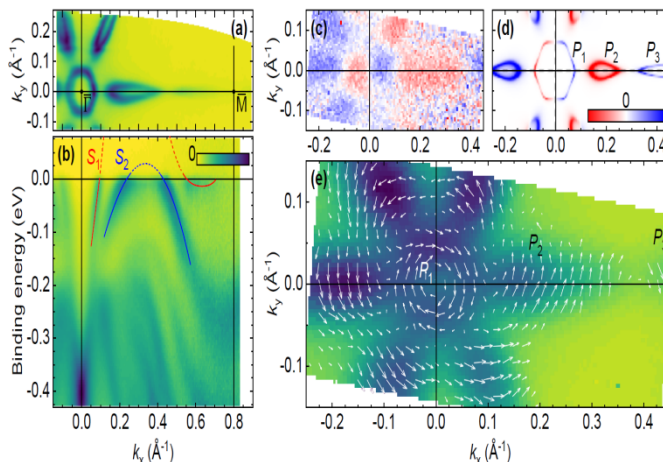
Fig.1. Spin-resolved surface states of a 5-nm \text{Bi}_{0.85}\text{Sb}_{0.15} on Si (1 1 1). (a) High-resolution ARPES at the Fermi energy (b) ARPES energy dispersion along the TM direction. The color bar represents the density of states in arb. units. (c) \sigma_y polarization DOS measured at the Fermi level where the color bar is proportional to the spin-polarization with scale extrema of P.S = \pm 0.1 ( T=300 K) and (d) corresponding TB modelling of the s-DOS projected on the first bilayer. The color bar indicates the spin polarization \sigma_y between -\sigma_{\max,y} \approx -0.7 and \sigma_{\max,y} \approx +0.7 . (e) Color map representing the measured ARPES intensity close to Fermi energy integrated on 25 meV with arrows representing the measured spin polarization direction and amplitude ( T=300 K). The different electron and hole pockets labeled P1, P2 and P3 in (d) are easily identified in the experimental measurements.
