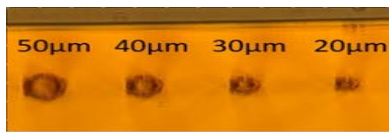
Fig. 1. End view of waveguides in Cr:ZnS crystal at \sim 200 \mu\text{m} depth (2090 nm writing). Laser beam is focused from above. Writing direction is perpendicular to the view plane. Since the index change in ZnS is negative, all waveguides are of depressed-cladding type, where the waveguide is formed by many lines of traces written around the unchanged core.
