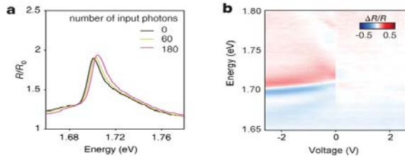
Fig. 1. Giant optical nonlinearity from exciton-hole interactions. a. Our results show strong oscillator strength and giant nonlinearity of Fermi polarons in trilayer WSe 2 , where hundreds of photons lead to a strong blueshift of the polaron resonance [Ref. 1]. b. Reflectance change induced by optical pumping in trilayer WSe 2 , showing drastically different behaviors in the hole vs. electron-doped regimes (negative vs. positive gate voltages).
