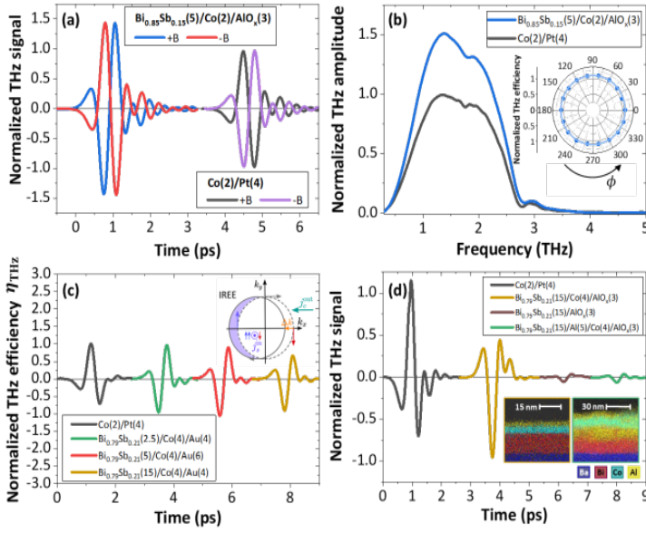
Fig.2. SCC and THz emission from \text{Bi}_{1-x}\text{Sb}_x/\text{Co} bilayers acquired at 300 K. (a) THz time-trace from \text{Bi}_{0.85}\text{Sb}_{0.15}(5)/\text{Co}(2)/\text{AlOx}(3) for \pm B compared to \text{Co}(2)/\text{Pt}(4) . (b) Spectral components of the THz emission from \text{Bi}_{0.85}\text{Sb}_{0.15}(5)/\text{Co}(2)/\text{AlOx}(3) and \text{Co}(2)/\text{Pt}(4) for +B . Inset) Normalized THz efficiency \eta_{\text{THz}} dependence on the azimuthal angle \phi . (c) THz efficiency as a function of the \text{Bi}_{0.79}\text{Sb}_{0.21} layer thickness (2.5, 5 and 15 nm) compared to \text{Co}(2)/\text{Pt}(4) . (d) THz signal \text{Bi}_{0.79}\text{Sb}_{0.21}(15)/\text{Al}(5)/\text{Co}(4)/\text{AlOx}(3) , \text{Bi}_{0.79}\text{Sb}_{0.21}(15)/\text{AlOx}(3) , \text{Bi}_{0.79}\text{Sb}_{0.21}(15)/\text{Co}(4)/\text{AlOx}(3) on \text{BaF}_2 and \text{Co}(2)/\text{Pt}(4) . Time traces are shifted in time for clarity. Inset) Fluorescence map obtained from a TEM cross-section \text{Bi}_{0.79}\text{Sb}_{0.21}(15)/\text{Co}(4)/\text{AlOx}(3) ( brown frame ) \text{Bi}_{0.79}\text{Sb}_{0.21}(15)/\text{Al}(5)/\text{Co}(4)/\text{AlOx}(3) ( green frame ) grown on \text{BaF}_2 .
