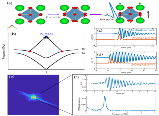
Fig. 1: Ionic Raman Scattering in SrTiO 3 . (a) Structure of STO and excitation scheme. The A 1g mode is illustrated in red ( center panel ) and the TO phonon at zone-center is illustrated on the right panel. (b) Schematic of the Ionic Raman scattering process in reciprocal space. Two TO phonons (red) combine and produce a single A 1g phonon (blue). (c) Predicted A 1g displacements based on a THz drive field (electronic Raman scattering). (d) Predicted A 1g displacements (blue) based on an ionic Raman scattering drive force (orange) for a single oscillating mode. (e) X-ray diffraction of a peak sensitive to octahedral rotation of the A 1g mode. (f) Time-dependent displacement of the A 1g mode. Note the slow buildup of amplitude over two cycles, indicating a resonant drive force.
