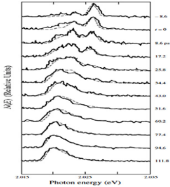
Fig. 1. Solid lines: time-resolved photoluminescence from excitons in Cu 2 O. Dashed lines: the results of a fit to the quantum Boltzmann equation for phonon emission and absorption. From[1].
