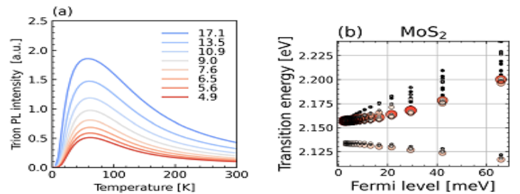
Fig. 1. Left: Temperature dependence of the photoluminescence trion peak in MoS 2 , where non-monotonic behavior is due to the low-lying dark trion states [2].
