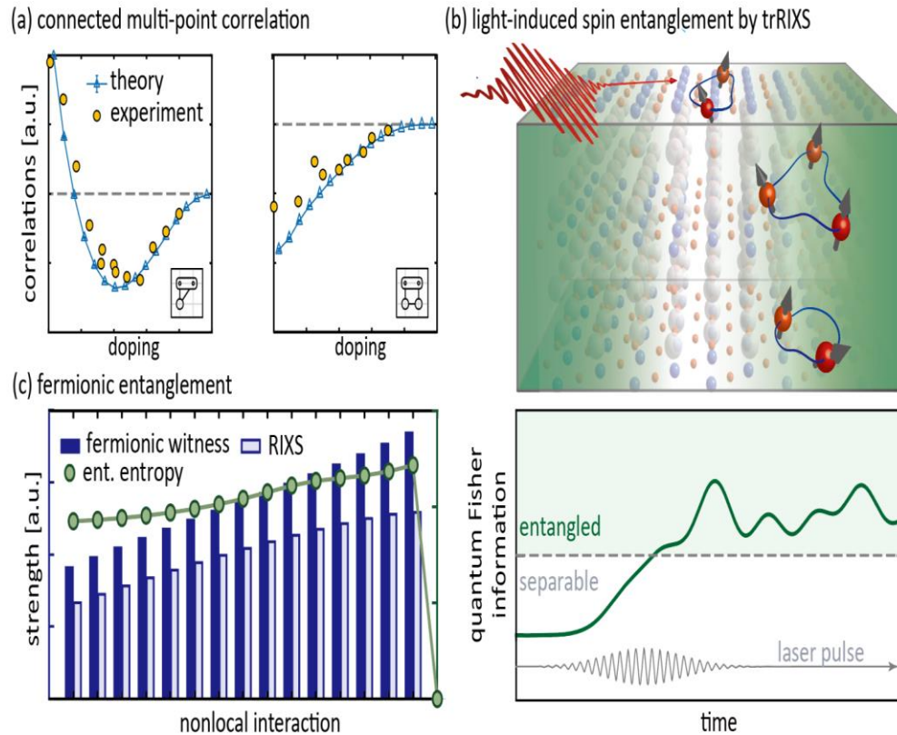
Fig. 1. (a). The simulated three-point (left) and four-point (right) correlations for doped Hubbard models, compared against the cold-atom experimental data (yellow circles). (b). Light-induced spin quantum Fisher information in a strongly correlated system, described by the single-band extended Hubbard model. The gray dashed line indicates the boundary between witnessed separable and entangled state. (c): fermionic entanglement witness extracted from RIXS spectrum, compared with the entanglement entropy. The simulation uses an extended Hubbard model as an example.
