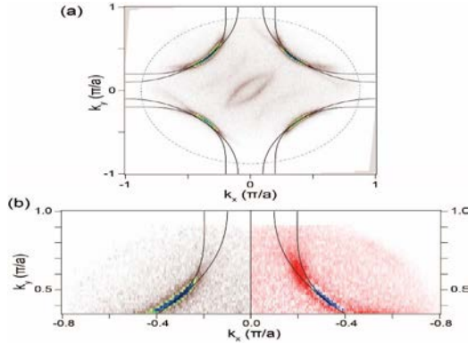
Fig. 1. (a): Fermi surface mapping of optimally-doped T_c \sim 91 K Bi2212. The solid lines show the bonding and antibonding bands. The dashed blue circle shows the momentum space that can be accessed using 6 eV photons. (b): photoexcited Fermi surface ( left ) and differential Fermi surface ( right ) at zero pump-probe delay upon 300 meV excitation.
