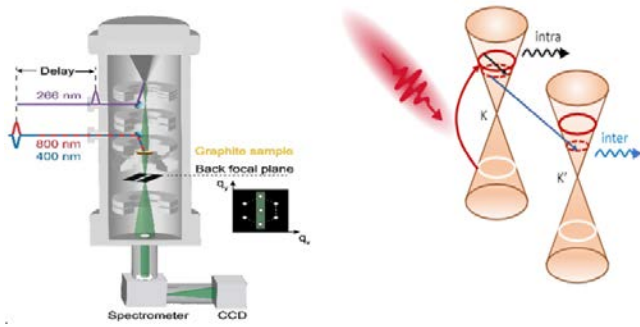
Fig. 1. Left: Experimental setup of momentum- and time-resolved EELS in an ultrafast TEM. Right: Sketch of the inter- and intravalley scattering processes for the relaxation of photo-excited electrons in graphite.
