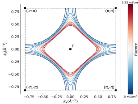
Fig. 2. Fluence-dependent Fermi-Surface evolution. Fermi-Surface is reconstructed from k_F points in a Tight-Binding approach
