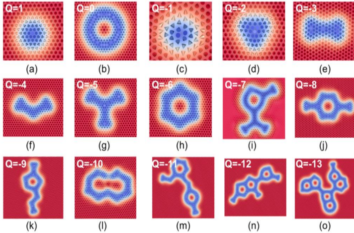
Fig. 1. A subset of identified topological metastable spin textures in the Pd/Fe/Ir(111) system with an external magnetic field of 3.5 T. (a) Skymion, (b) skymionium, (c) antiskyrmion, (d)–(o) isolated magnetic textures, with higher-order topological charge varying between Q = -2 and Q = -13 . The distance between neighboring Blue and red colors indicate opposite spin directions.
