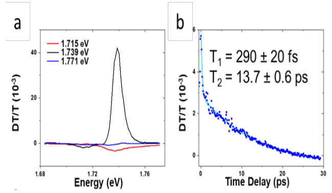
Fig.3 Differential transmission induced by pump divided by transmission without pump ( \text{DT}/T ). (a) Frequency dependence for three different pump frequencies. (b) Time dependence for pump frequency of 1.736 eV showing ultrafast (290 fs) initial recovery. [1].
