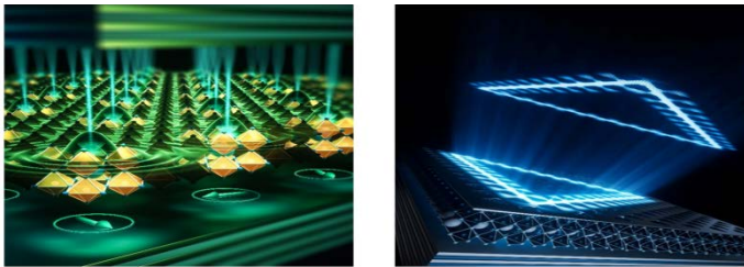
Fig. 1. Left: Schematic of polaritonic XY spin Hamiltonian Right: Schematic of polaritonic valley Hall laser.
