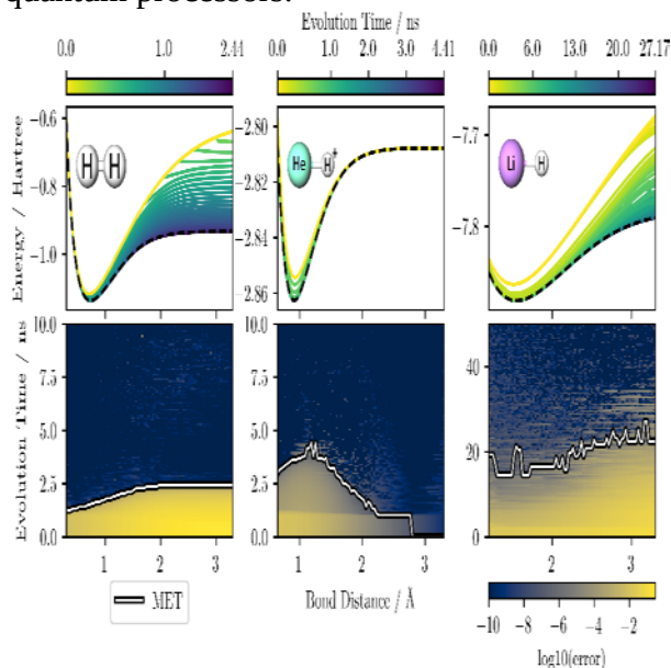
Fig. 1. Estimates of the disassociation curves for H_2 (left), HeH^+ (centre), and +LiH (right). For each molecule and bond separation the numerically simulated silicon quantum processor is given a fixed amount of evolution time as a resource and prepares the best possible approximation to the ground state in this time. As more time is allowed, the quantum processor can obtain better approximations. The top three panels plot the disassociation curves (energy against bond separation), with the colour of the curve corresponding to the allowed evolution time indicated by the colour bar above each panel. The yellow curve corresponds to zero evolution time. The purple curve corresponds to enough time to reach the full configuration interaction (FCI) energy (dashed curve). In the bottom panels, the error from the FCI energy is plotted on a log scale with the evolution time now on the vertical axis. In the bottom panels, we observe a sharp transition: above an evolution time called the minimal evolution time (MET), the ground state can be prepared exactly. We indicate the MET as a function of bond distance by a black-and-white curve. Below the MET, the error is large, and the corresponding colour is yellow, as indicated by the bottom right colour bar. While above the MET, the error is small and fluctuates around the simulation accuracy, and the corresponding colour is blue.
