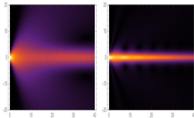
Fig. 1. Modeling of laser radiation propagation bio-suspension in (x,z) plane at different initial field amplitudes : Left: initial field amplitude is less than threshold for self-channeling regime; Right: initial field amplitudes is more than threshold for self-channeling regime.
