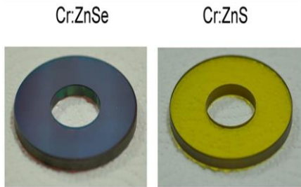
Fig. 1. Ø50x5mm Cr:ZnSe and Cr:ZnS gain elements with Cr concentration 10^{19}
