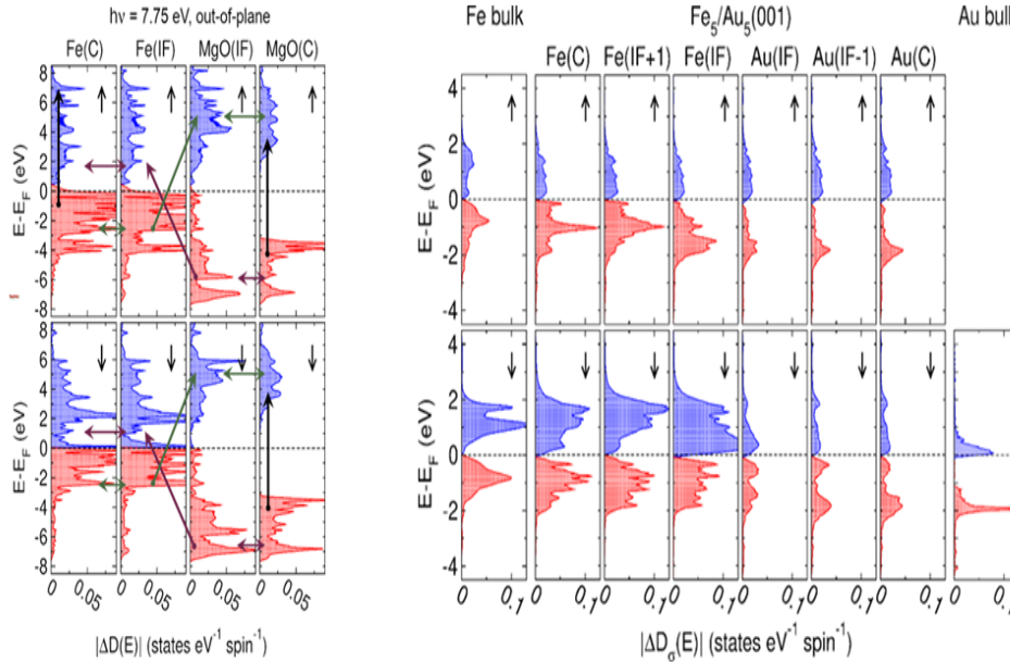
Fig. 1. Spin- and layer-resolved changes in the density of states \Delta D(E) = D_\sigma(E, 20\text{fs}) - D_\sigma(E, 0) Left: of the central and interface layers of Fe and MgO in \text{Fe}_5/(\text{MgO})_7(001) , excited with an out-of-plane laser pulse with h\nu = 7.75 eV. Purple and green arrows indicate concerted transfer and excitation of carriers. Adapted from Ref. [3]; Right: in a \text{Fe}_5/\text{Au}_5(001) heterostructure and bulk Fe and Au. Adapted from Ref. [4]. Blue: positive sign, accumulation; Red: negative sign, depletion of occupation. The upper panels refer to the majority spin channel and the lower panels to the minority spin channel.
