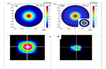
Fig. 4. Intensity I profiles of the amplified field after 3.4 cm Cr:ZnS waveguide of 50 \mu\text{m} (a), and 20 \mu\text{m} (b) diameters. The input energy of the 500 ps seed pulse is 1.47 nJ and the pump powers are 22 W (a) and 12 (b) W. Inset in (b) shows the field profile after 3.28 cm propagation distance in a waveguide. G is a gain factor (arb.un.). (c) and (d): output beam profiles for 50 \mu\text{m} (c), and 20 \mu\text{m} (d) waveguide diameters.
