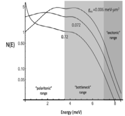
Fig. 2. The steady-state distribution of polaritons in a microcavity for three different choices of exciton-exciton interaction strength. From[3].
