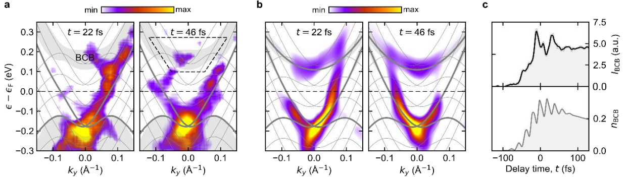
replicas. c) Experimental (upper panel) and theoretical (lower panel) temporal evolution of the photoelectron intensity integrated across the bulk conduction band (dashed trapezoid in a)
