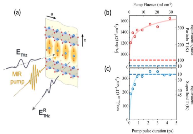
Fig. 1. a- Schematic of the mid-infrared (MIR) pump-THz probe experiment in \text{YBa}_2\text{Cu}_3\text{O}_{6.48} . The sample is excited by a MIR pump pulse (yellow) polarized along the crystal c -axis, resonantly driving apical oxygen phonon modes as indicated inside the yellow shading. The subsequent changes in the low-frequency optical properties are sampled by a broadband, also c -polarized THz probe pulse (grey). b- Evolution of the transient spectral weight and (c) of the coherent superconducting-like response measured at the time delay corresponding to the peak of the light-induced response, as a function pump pulse duration. The top horizontal axis indicates the pump fluence which increases linearly with the pump pulse duration to keep the peak electric field constant. The red and blue horizontal dashed lines in (b) indicate the equilibrium spectral weight values at T = 100 K and T = 10 K, respectively, while that in (c) refers to the equilibrium superfluid density at T = 10 K. Equivalent temperatures are reported on the right axes.
