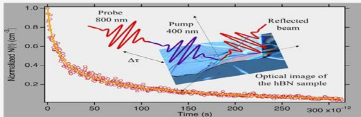
Fig.1. The graph displays the normalized differential transients plotted as a function of the time delay between the pump and probe pulses. The yellow solid line represents the fit of the data. The inset shows the sample and illustrates the pump-probe principle.
