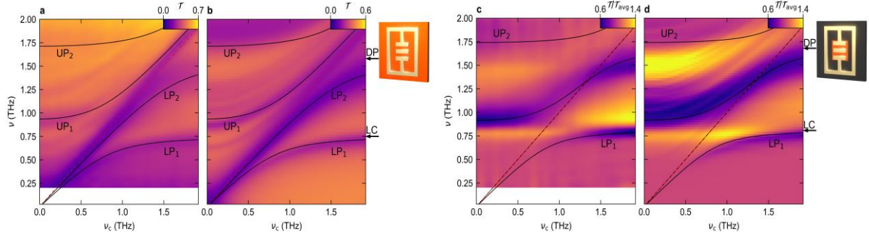
Fig. 2 a. Experimental transmission spectra of the unstructured sample as a function of the cyclotron frequency \nu_c . The curves represent the eigenmodes calculated by theoretical fit. b. FEFD simulation of the transmission spectra of the structure including the theoretical fit of panel a . The two arrows indicate the frequencies of the uncoupled LC and DP modes obtained by our fit. Outset: Schematic of the resonator on top of an unstructured QW (bright orange area). c. Experimental transmission spectra of the unstructured sample, each normalized to the average transmission \nu_g for each frequency \nu , as a function of \nu_c . The curves represent the eigenmodes calculated by theoretical fit. d. FEFD simulation of the transmission spectra of the structure, each normalized to the average transmission T_{avg} for each frequency \nu as a function of \nu_c , including the theoretical fit of panel a . The two arrows indicate the frequencies of the uncoupled LC and DP modes obtained by our fit. Outset: Schematic of the resonator on top of a structured QW patch (bright orange patch).
