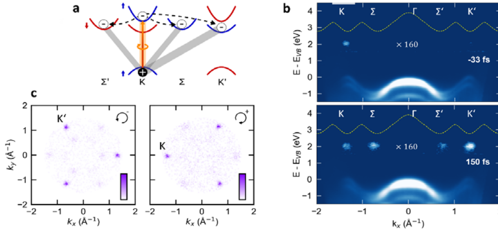
Fig. 1. a: Energy scheme of WS 2 with bright and momentum-dark excitons.
