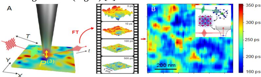
Fig. 2. (A) Ultrafast nano-imaging of photoinduced polaron dynamics in triple cation perovskites. (B) Ultrafast movie resolving heterogeneity in carrier dynamics and polaron radius underlying the performance of perovskite-based photophysical devices of solar cells, lasers, and light emitting diodes.
