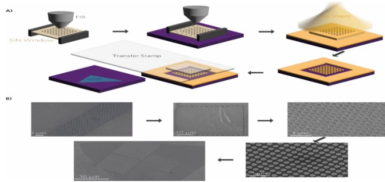
Fig. 1. An illustration of the fabrication steps with the corresponding SEM/FIB images. A , A commercial \text{SiN}_x membrane is milled, flipped, and lowered to contact the substrate. The window is removed, and the material of choice is evaporated. The membrane is loosely stuck to the surface and can be easily removed with a low-adhesion tape. After the removal, the nanostructures can be transferred onto the sample of interest. B , Clockwise, from top right : Milled membrane (SEM); the sides are cut with FIB (FIB); before the membrane is removed (SEM); after the nanostructures are transferred on a single-layer \text{WSe}_2 sample (SEM).
