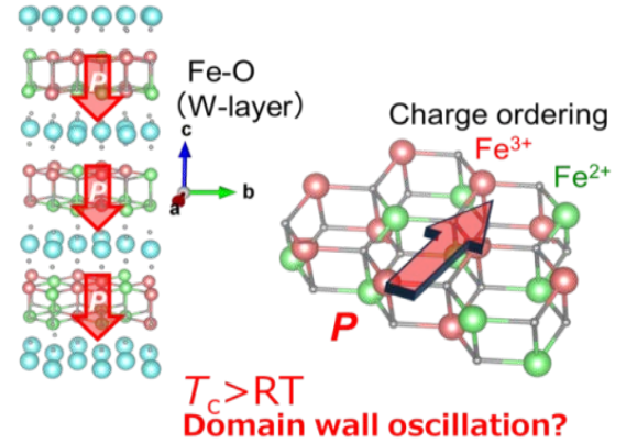
Fig. 2 Crystal structure and ferroelectric CO in \text{LuFe}_2\text{O}_4
