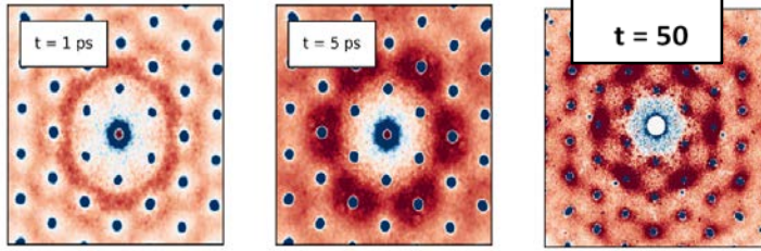
Fig. 1. a-c. Momentum-resolved electron diffraction signals, I(q, t) - I(q, t < t_0) , at pump-probe delays of 1, 5, and 50 ps. The Bragg reflections (blue dots) are negative due to the Debye-Waller effect. The diffuse background (red) qualitatively evolves as a function of pump-probe delay. The inelastic signals at 5 ps qualitatively depart from the non-thermal signals at 1 ps and quasi-thermal signals at 50 ps. This indicates that MoS 2 undergoes two qualitatively distinct non-thermal phonon populations before the lattice reaches a hot but thermal state.
