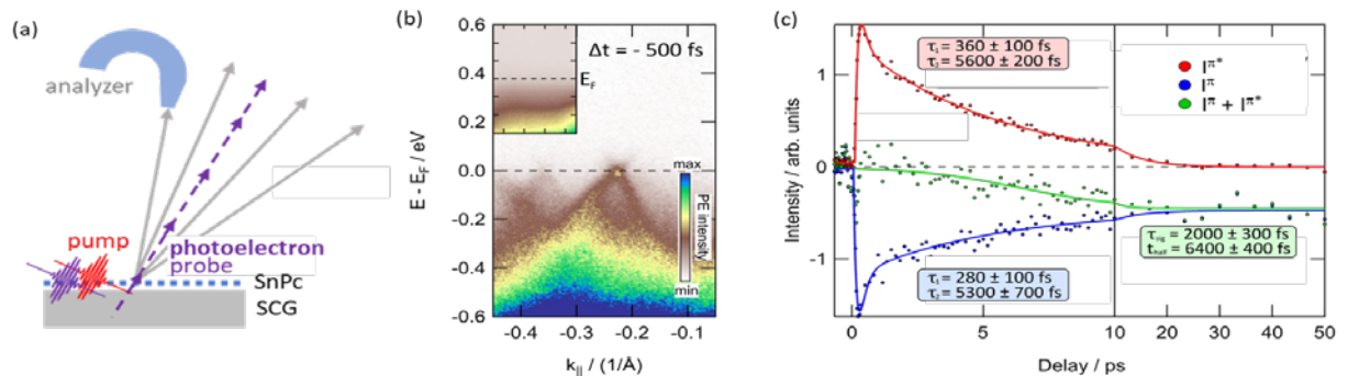
Fig. 1. (a) Experimental scheme for ULEPD. (b) ULEPD signal of SnPc/graphite 500 fs before photoexcitation. The inset shows the same energy-momentum field of view for the pristine graphite sample. (c) ULEPD transients extracted from energy regions above (red) and below (red) E_F . The green data results from the sum of these transients and represent structural changes in the adsorbate layer due to vibrational disorder. Lines are fits to the data.
