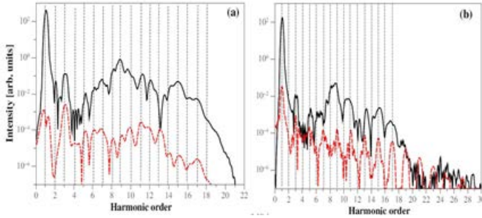
Fig. 1. Power spectrum of intra- (dashed red line) and inter-band (solid black line) currents in the bulk of ZnO for peak laser intensity 10^{12} \text{ W/cm}^2 , laser wavelength 3 \mu\text{m} and pulse duration of 60fs.
