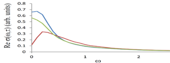
Fig. 1. Time-dependent optical conductivity excited by pump pulses for a four-hole doped two-leg ladder Hubbard lattice with 16 \times 2 = 32 sites and on-site Coulomb interaction U=10 in the unit of hopping energy. The amplitude of the vector potential is set to be A_0=0.5 . Blue line is for time \tau < 0 (before pumping). Red line represents spectrum for a monocycle pulse with pump frequency \omega_p=0 calculated at time \tau=12 when pump pulse is finished. Green line is for a pump pulse with \omega_p=1 .
