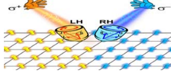
Fig. 1. Circularly left ( \sigma^+ ) and right ( \sigma^- ) polarized laser pulses induced chiral dynamics in 2D ferromagnets.
