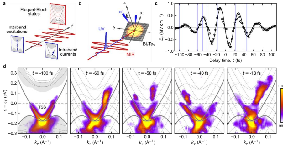
Fig. 1: a) Transition between subcycle dynamics and quasi-static Floquet-Bloch bands. b) Experimental scheme: an s-polarized, phase-stable MIR pulse (red) drives the topological surface state (TSS) of \text{Bi}_2\text{Te}_3 . An ultraviolet (UV) probe pulse (blue) at variable time delay, t , provides snapshots of the induced dynamics with subcycle temporal resolution.
